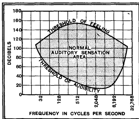
Fig. 1. Diagram showing thresholds of audibility and feeling for normal ears.
