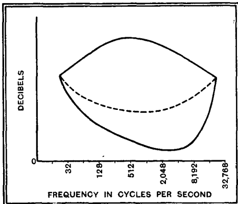
Fig. 2. The dotted line shows the threshold of audibility of a person who is equally deaf over the frequency range.
