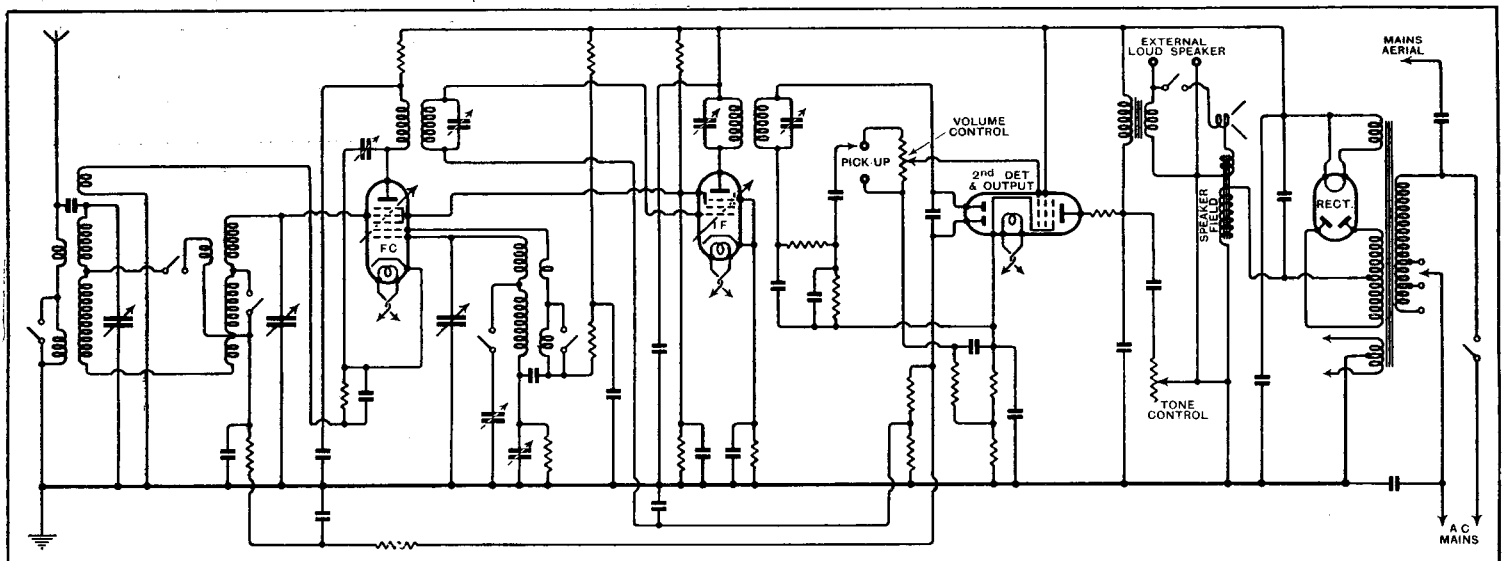
Complete circuit diagram. An image suppressor circuit is included in the input band-pass filter, which employs "mixed" coupling.
