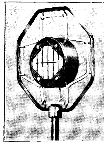
T.M.C. Varidep transverse current microphone embodying some new features.
