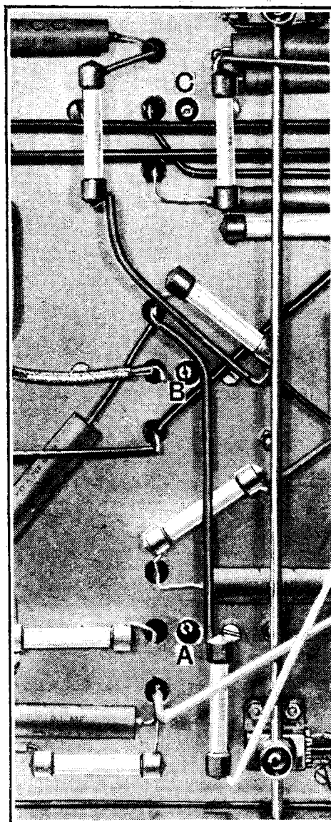
In this view of the receiver the secondary IF transformer trimmers can be seen and are again lettered A, B, and C for the 1st, 2nd, and 3rd transformers.
