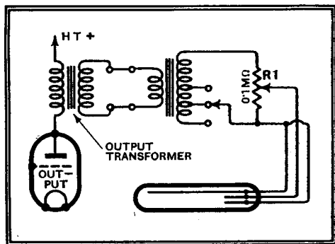
Fig. 1.—Explaining the use of a neon tuning indicator as an output meter.
