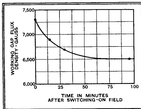
Fig. 1.—Showing time-flux relationship for energised magnet.
