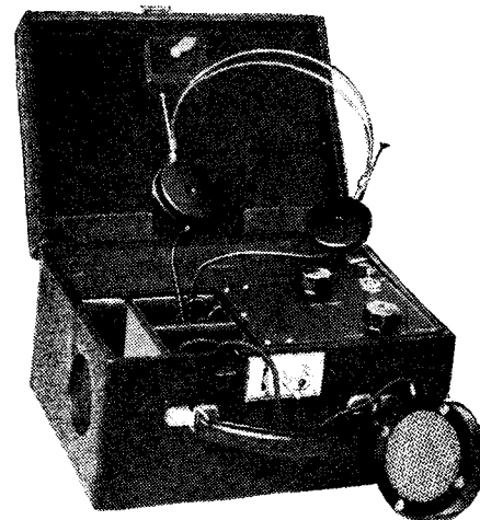
Fig. 14. Multitone Electric portable valve-type deaf-aid.
