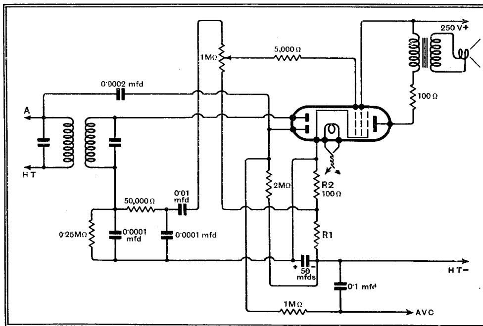
Fig. 2.—Typical connections for a duo-diode output pentode are given here. The AVC delay voltage is governed by the value of R1.
