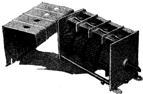
Polar four-gang Midget condenser.
