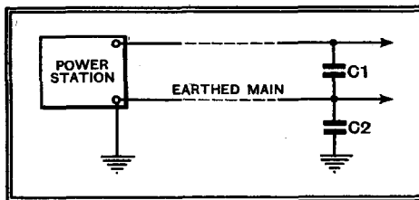
Fig. 2.—Explaining how the filter of Fig. 1 (b) avoids leakage to earth of AC.
