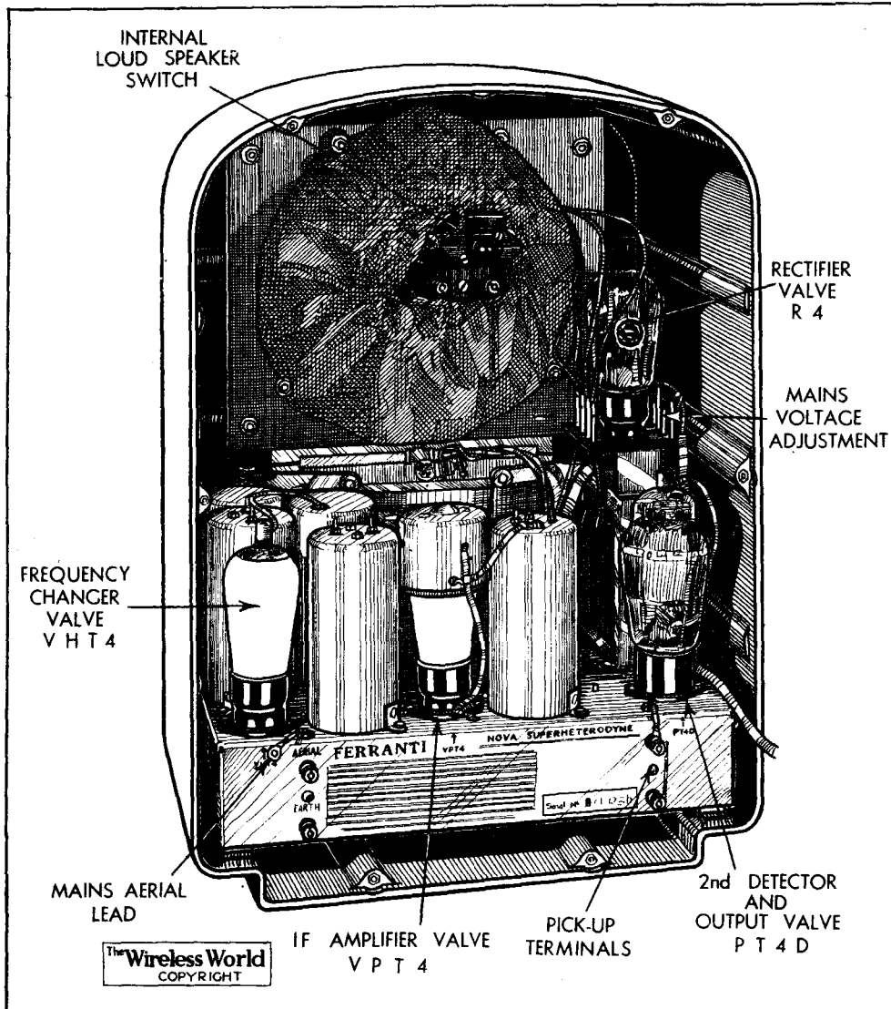
Lightness and strength are combined in the moulded bakelite cabinet. For gramophone reproduction the flexible lead attached to one of the pick-up terminals is removed.
