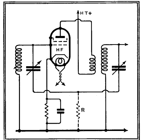
Fig. 1.—How defective earthing of a ganged condenser causes instability.
