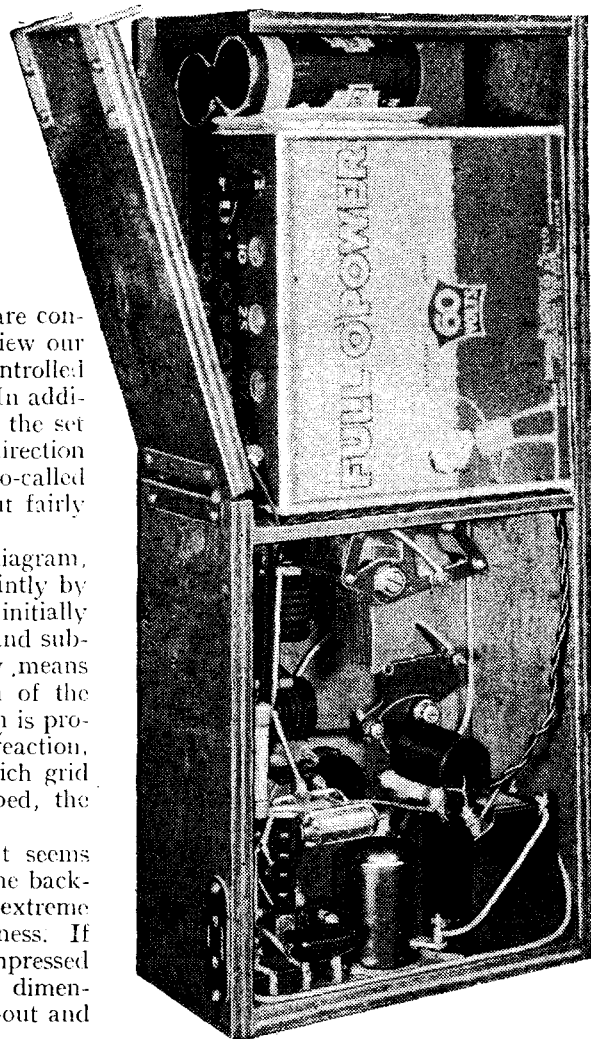
Showing the hinged flap which allows easy access to the LT battery for replacement.
