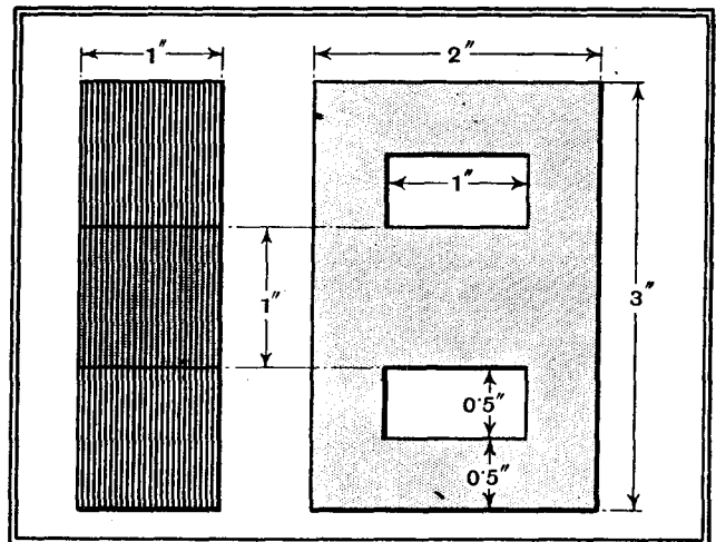
Fig. 2. Dimensions of core assumed in the worked example.
