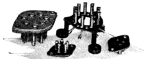
Clix valveholders for short-wave use and for the Hivac pin-type Midget valves.
