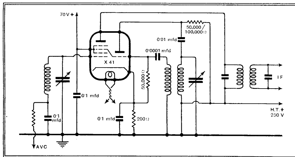
Fig. 1.—The recommended circuit connections for the triode-hexode frequency-changer are shown here. A tuned-anode oscillator circuit is advised for the best results.
