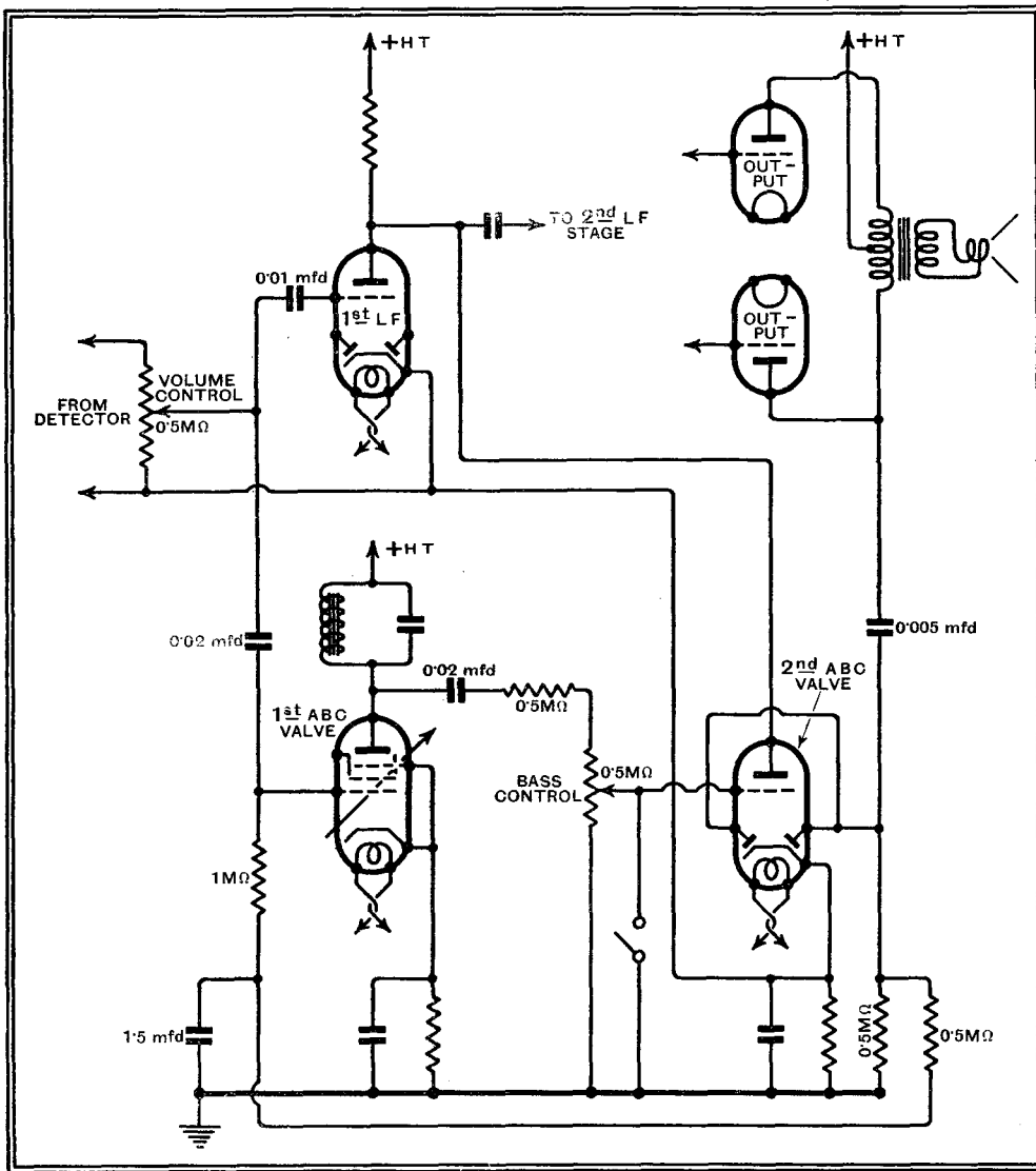
Fig. 3.—Skeleton circuit diagram of an "automatic bass compensation" system. The two lower valves are the additional ones required.
