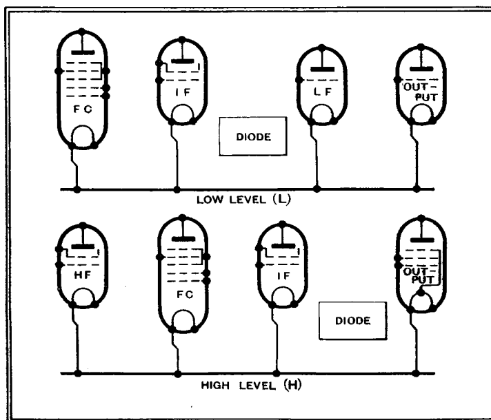
Fig. 1.—Typical functions of valves in small superhets with low-level and high-level detection; the diode detector is usually combined with one of the amplifying valves.
