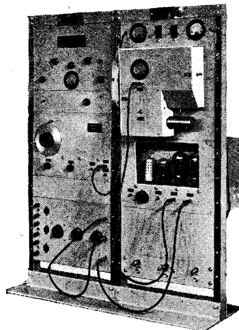
Complete loud speaker calibrating equipment built on the rack system and shown by Tannoy Products.
