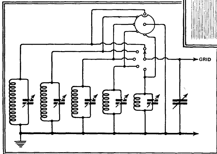
Fig. 1.—The ideal switching arrangements for one circuit of an all-wave receiver are shown here. The lower switch selects the desired coil and the upper short-circuits all others.
