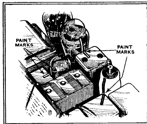
Fig. 2.—Guide marks as an aid to the correct insertion of valves.
