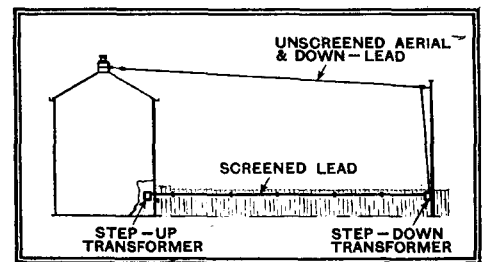
Fig. 6.—A screened lead-in with unscreened download.
