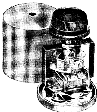
Colvern variable selectivity 465 kc/s IF transformer.
