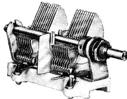
Polar dual short-wave condenser, Type E.
