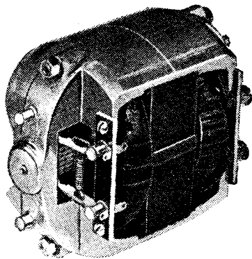
Redesigned Electro Dynamic car radio 12-watt HT rotary transformer.
