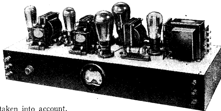
Ferranti Constructors Amplifier, Type AC6C, which provides sufficient magnification for operation with a microphone.
