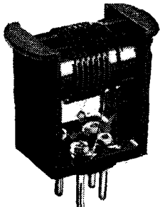
The new Colvern short-wave coils are fitted in a cradle-type carrier to ensure short low-capacity leads.
