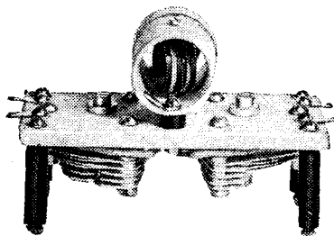
B.T.S. 12 Mc/s IF transformer for ultra-short wave superheterodynes.
