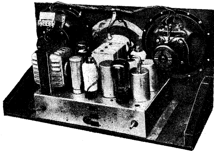
Chassis of the C.A.C. Austin AC Super Six.
