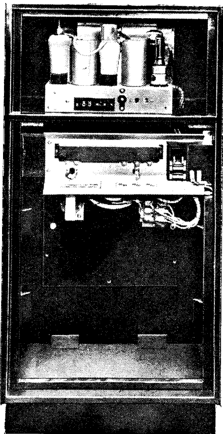
Rear view of H.M.V. universal console.
