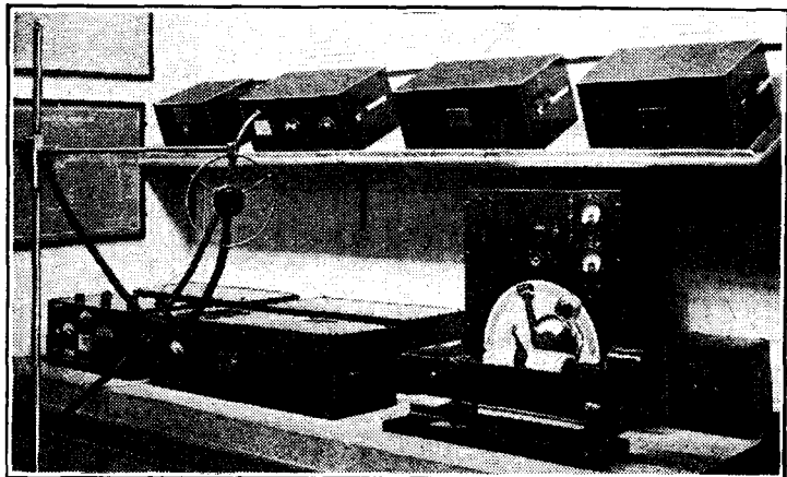
Laboratory apparatus used for measuring the response curves of Magnavox (Benjamin) loud speakers.
