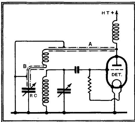
Fig. 2.—The stray capacity introduced by screening reaction leads is seldom harmful.
