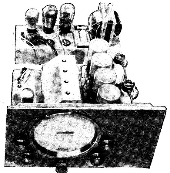
Chassis of the Dynatron Ether Knight.
