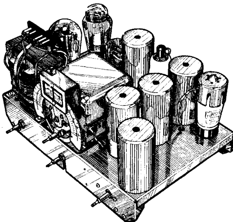
"The thoroughness of the workmanship can usually be judged by the exterior of the chassis." This drawing is of the chassis of one of the Murphy receivers.
