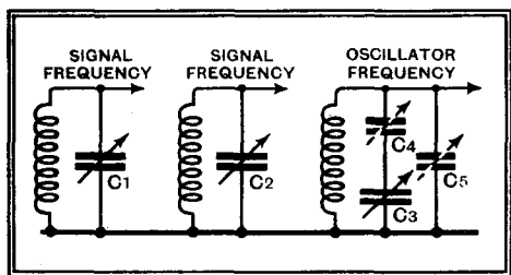
Fig. 1.—Single-knob tuning of a superheterodyne with a plain three-gang condenser.
