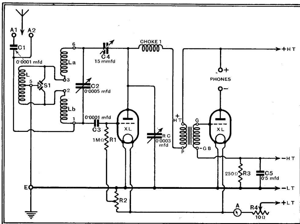
Complete circuit diagram. The medium-wave coil, which is interrupted at its centre point, comprises the windings La and Lb. The long-wave coil is marked L.
