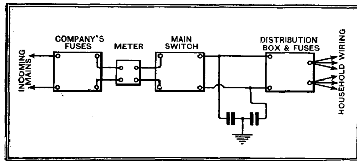
Fig. 3.—Diagrammatic sketch showing a convenient position for a mains input filter.
