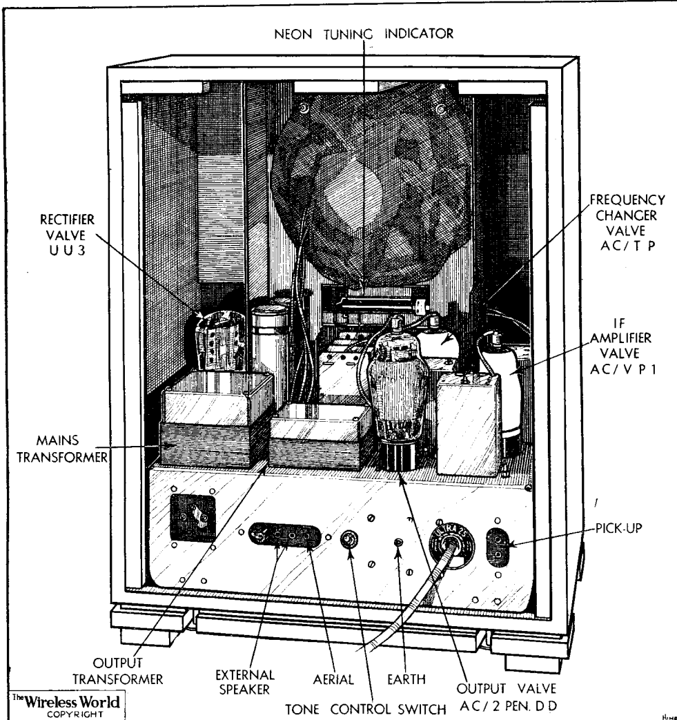
The loud speaker unit in the Ultra 25 is incorporated in the metal chassis framework.
