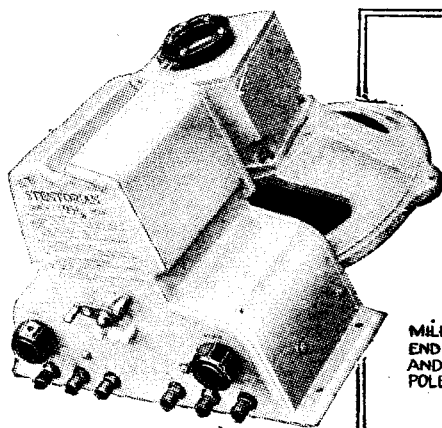
Whiteley "Stentorian Duplex" partly dismantled showing tweeter diaphragm. Note independent volume controls and output terminals. (Right) A section of "Stentorian Duplex" magnet system.
