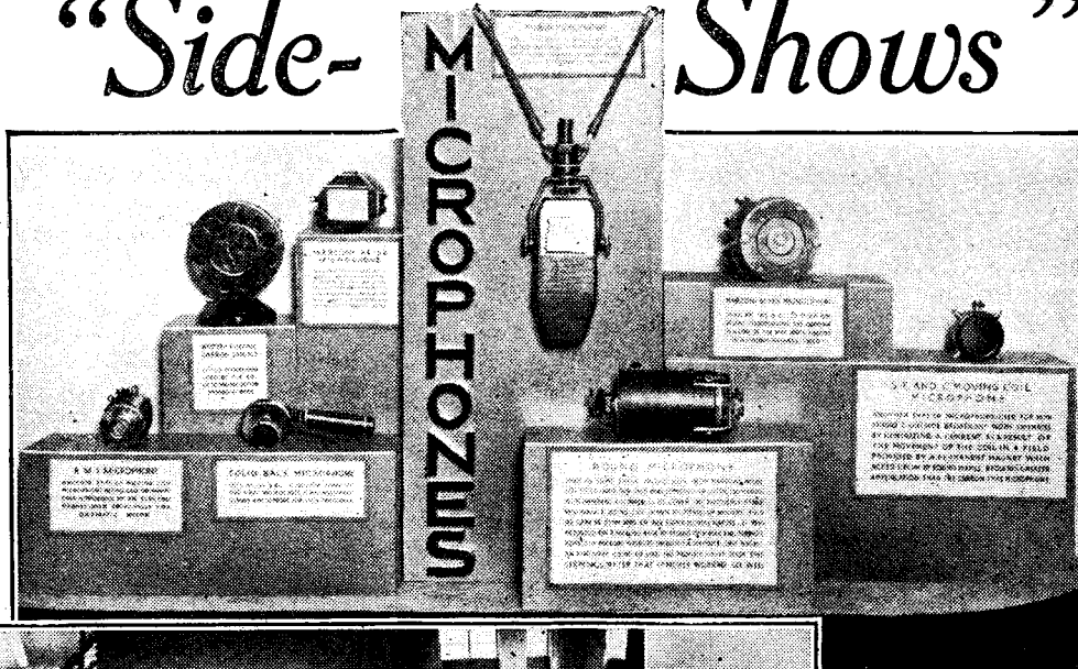
Microphones ranging from the solid-back type of 1923 to the "ribbon mike" of to-day are seen above in a photograph taken on the B.B.C.'s stand. On the left is a section of the photo-mural showing the technical side of the Corporation's work. Exterior and interior views of the Droitwich station can be picked out. The National and Midland transmitters are in the centre.
