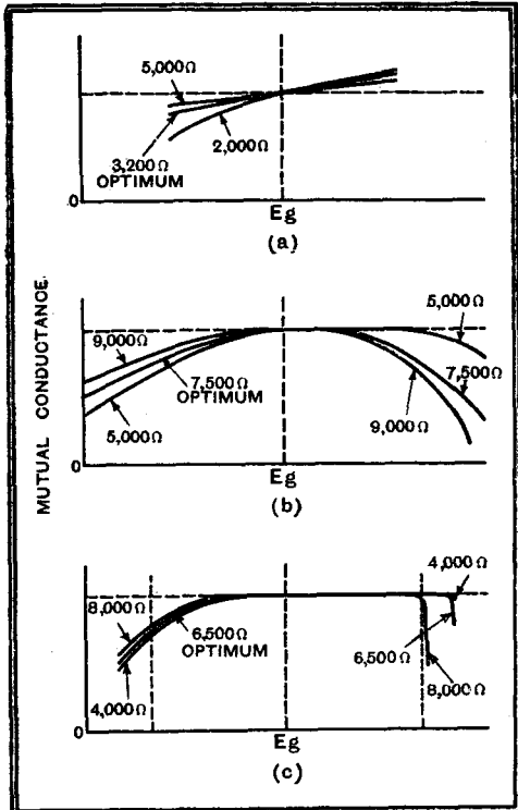
Fig. 4.—The variation of mutual conductance with input grid volts for a triode, a pentode and a Harries valve. The curves correspond to the load values marked.
