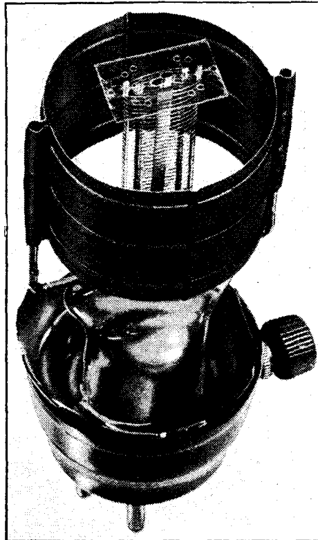
The feature of the valve is the abnormal spacing between the anode and outer grid.
