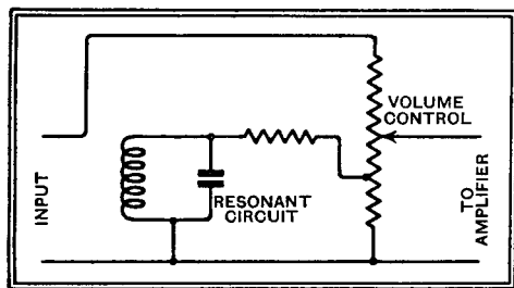
Fig. 1.—Circuit of a simple type of tone-compensated volume control.
