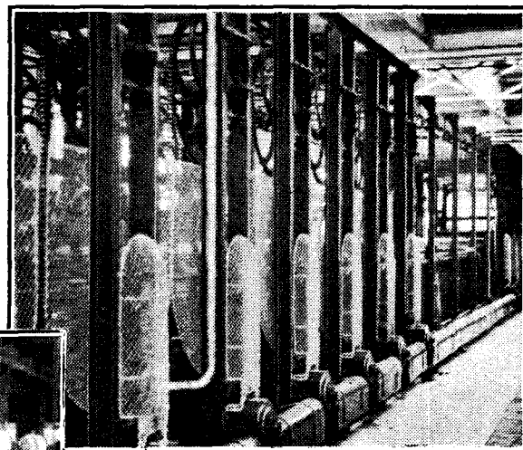
(Left) Receiving stores for raw materials. (Right) Automatic cadmium plating plant. (Below) A battery of light presses in the machine shops. Note the independent driving motors.
