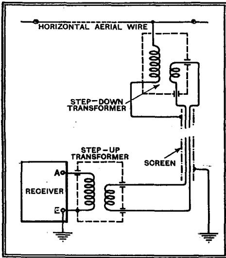
Fig. 5.—The theory of the transmission line download.
