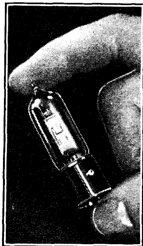
Hivac Midget Valve with base for bayonet socket; a pin-type base is also made.
