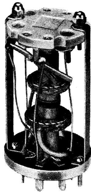
Bulgin variable selectivity 450 kc/s IF transformer
