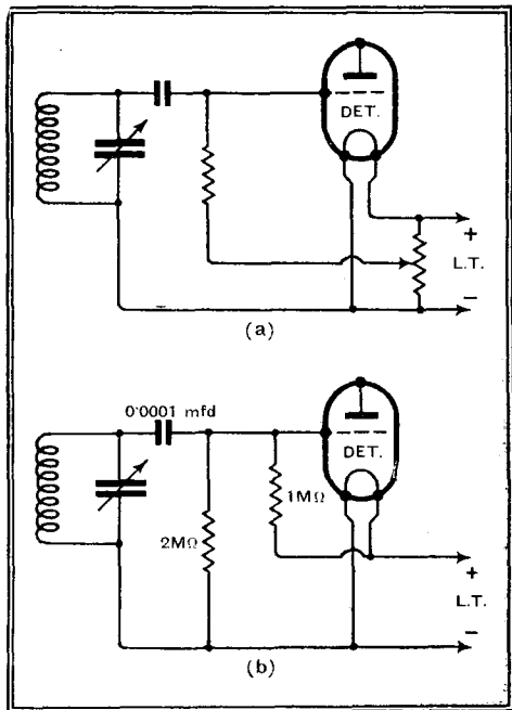
Fig. 1.—Two methods of improving the smoothness of reaction control.
