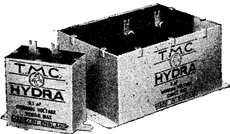
T.M.C.-Hydra condensers for use in high-voltage circuits.
