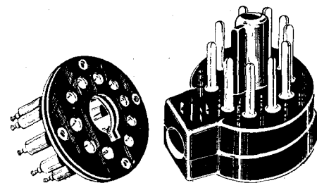
One of the new Belling-Lee components, a safety-type 10-pin cable plug and socket.
