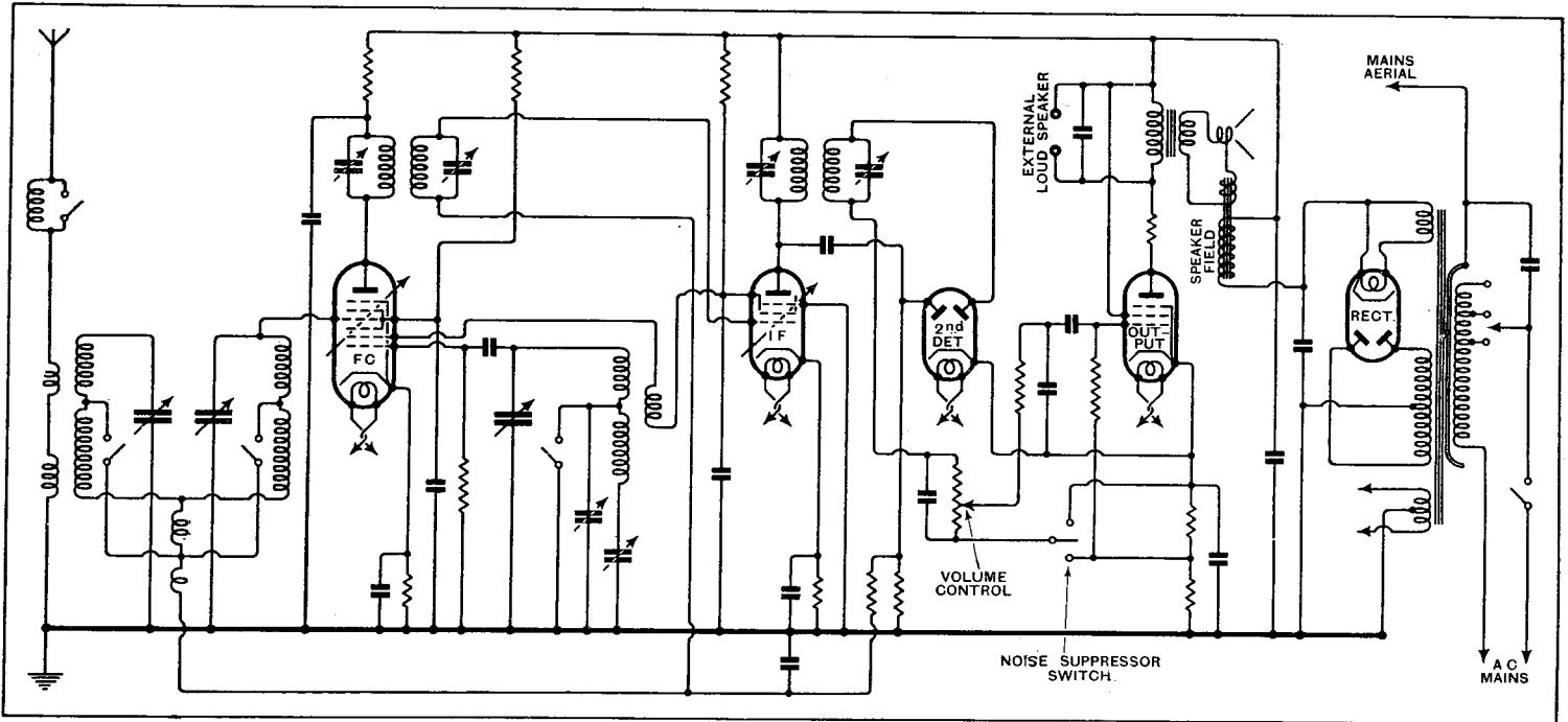
The aerial input and AVC circuits have been specially designed to give uniform sensitivity over both medium- and long-wave ranges.
