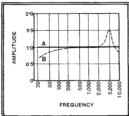
Fig. 1.—An ideal response curve compared with one having a pronounced peak as about 5,000 c.s.
