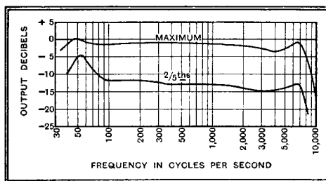
Fig. 2.—Characteristics of simple tone-compensated volume control, showing effectiveness of bass reinforcement.
