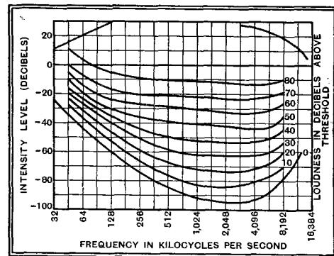
Fig. 5.—Diagram showing the intensities of sound required to give various degrees of loudness judged by a normal ear.
