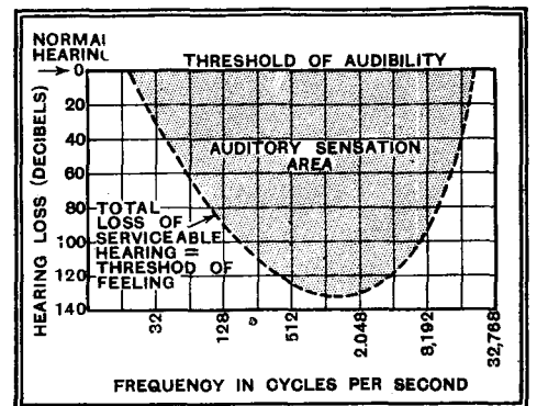
Fig. 5. Showing Fig. 1 plotted in a different manner which is suited to plotting measurements on deafness. The shaded areas are equal in both cases, as also are the vertical distances between the curves at the corresponding frequencies. Audiograms are always given in this form.
