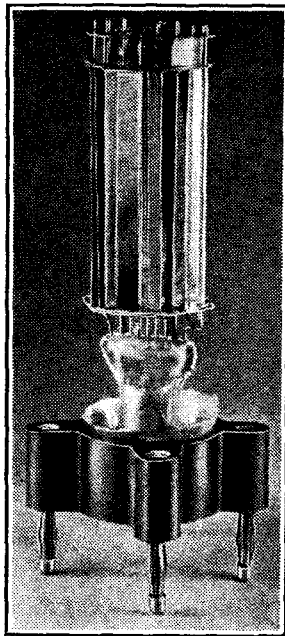
Interior of the 362 PX50 valve.
