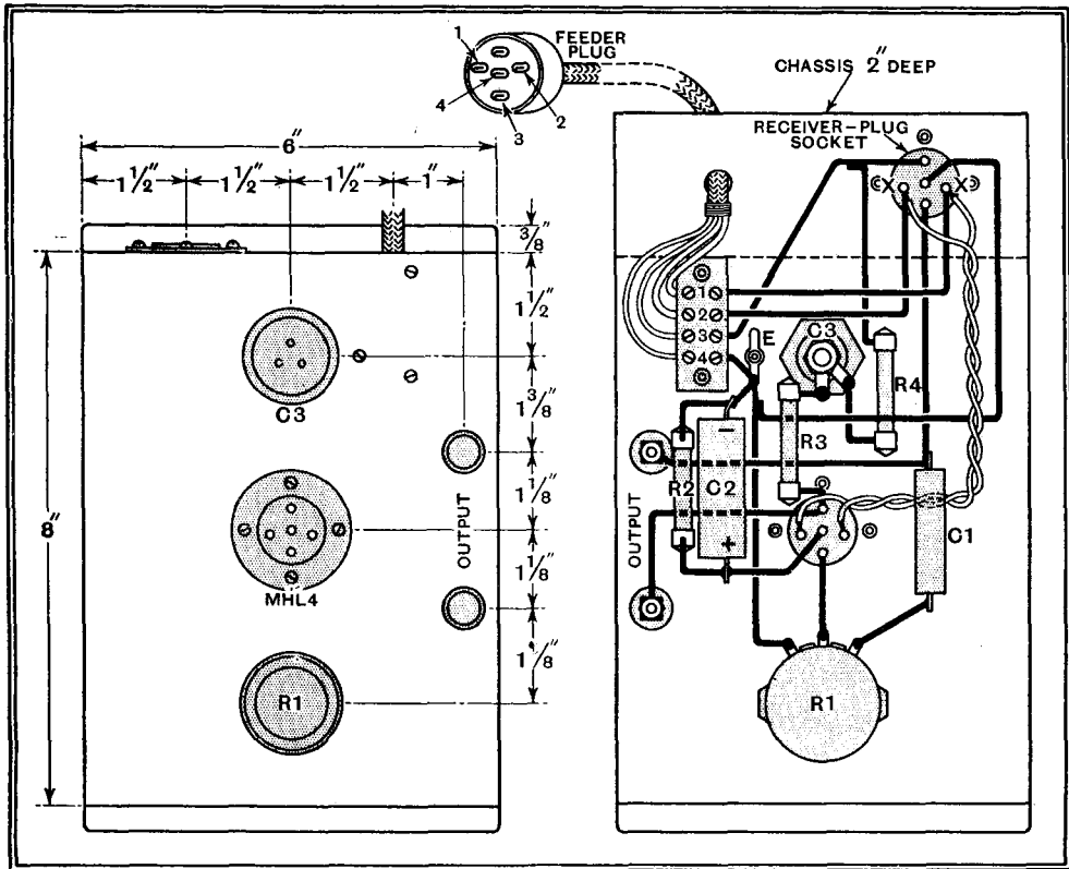
The construction and wiring are clearly shown in these drawings.
