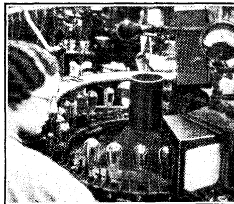
Exhausting machine. The final trace of gas is removed by igniting a small quantity of magnesium inside the bulb by means of a high-frequency induction coil.
