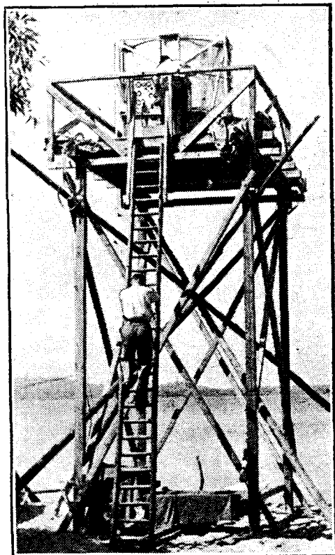
The micro-wave beacon projecting an invisible beam across the lake.
