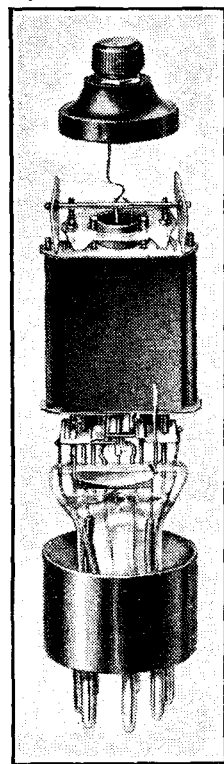
The Osram A537 special "noiseless" triode for microphone amplifiers is fitted with a top-cap for the grid connection. Steatite insulation is used.
