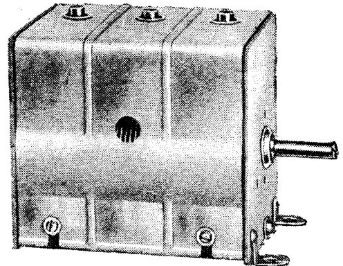
Polar midget three-gang superhet condenser.
