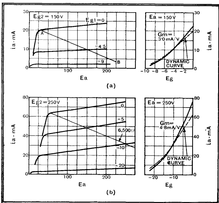
Fig. 2.—The characteristics of the new two-volt battery operated valve and of the new mains type valve.
