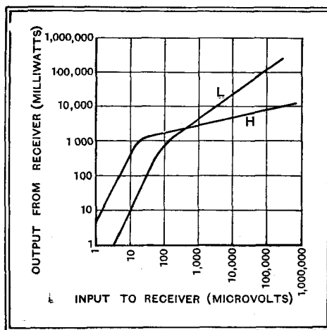
Fig. 2.—Outputs of low-level and high-level detector sets compared.
