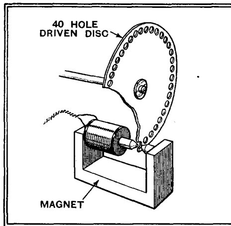
Fig. 1.—A thin metal disc mounted on the motor spindle and revolving between the poles of a magnet is used to generate the higher frequencies.
