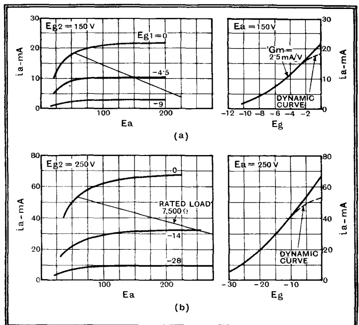
Fig. 3.—The characteristics of a two-volt pentode and a mains pentode exactly equivalent to the new valves shown in Fig. 2.
