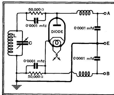
Fig. 2.—Method of feeding a push-pull amplifier from a diode detector, which allows one side of the circuit LC to be earthed.
