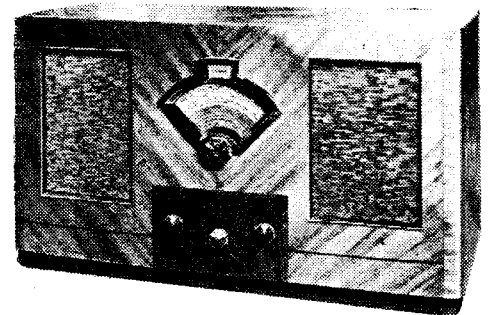
The C.A.C. Austin AC Super-Six.
