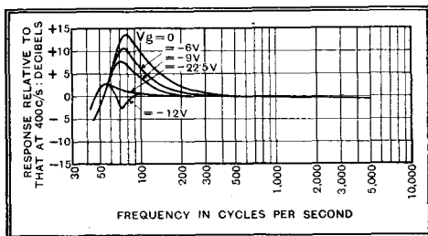
Fig. 4.—Characteristics of automatic bass compensation. The V_g figures are the controlling grid bias to the first A.B.C. valve derived by rectifying the signal potentials obtained from the output stage.
