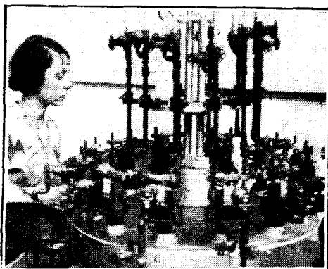
(Above) Rotary machine for forming valve pinches. (Left) Vacuum furnaces for extracting gas and cleaning electrodes before assembly.
