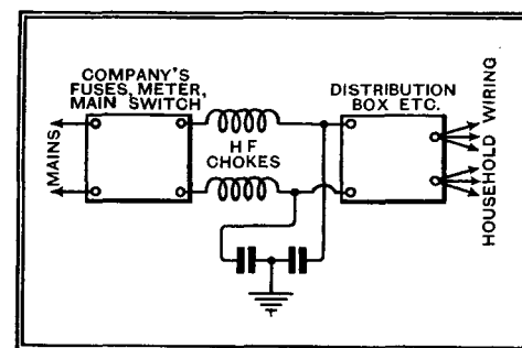
Fig. 4.—A choke-condenser filter; it is sometimes advantageous to transfer the condenser to the other side of the chokes.
