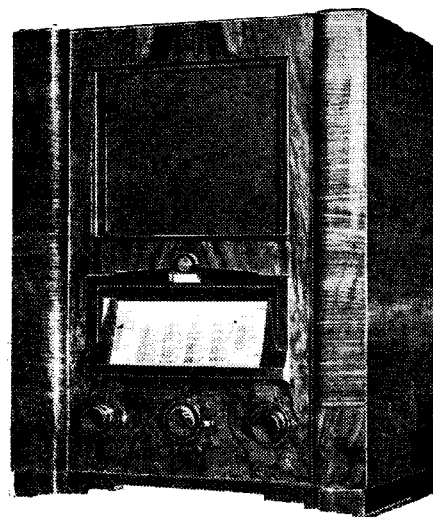
The Philips receiver has a signal-frequency HF stage and covers 16/50 metres as well as the medium and long wavebands.
