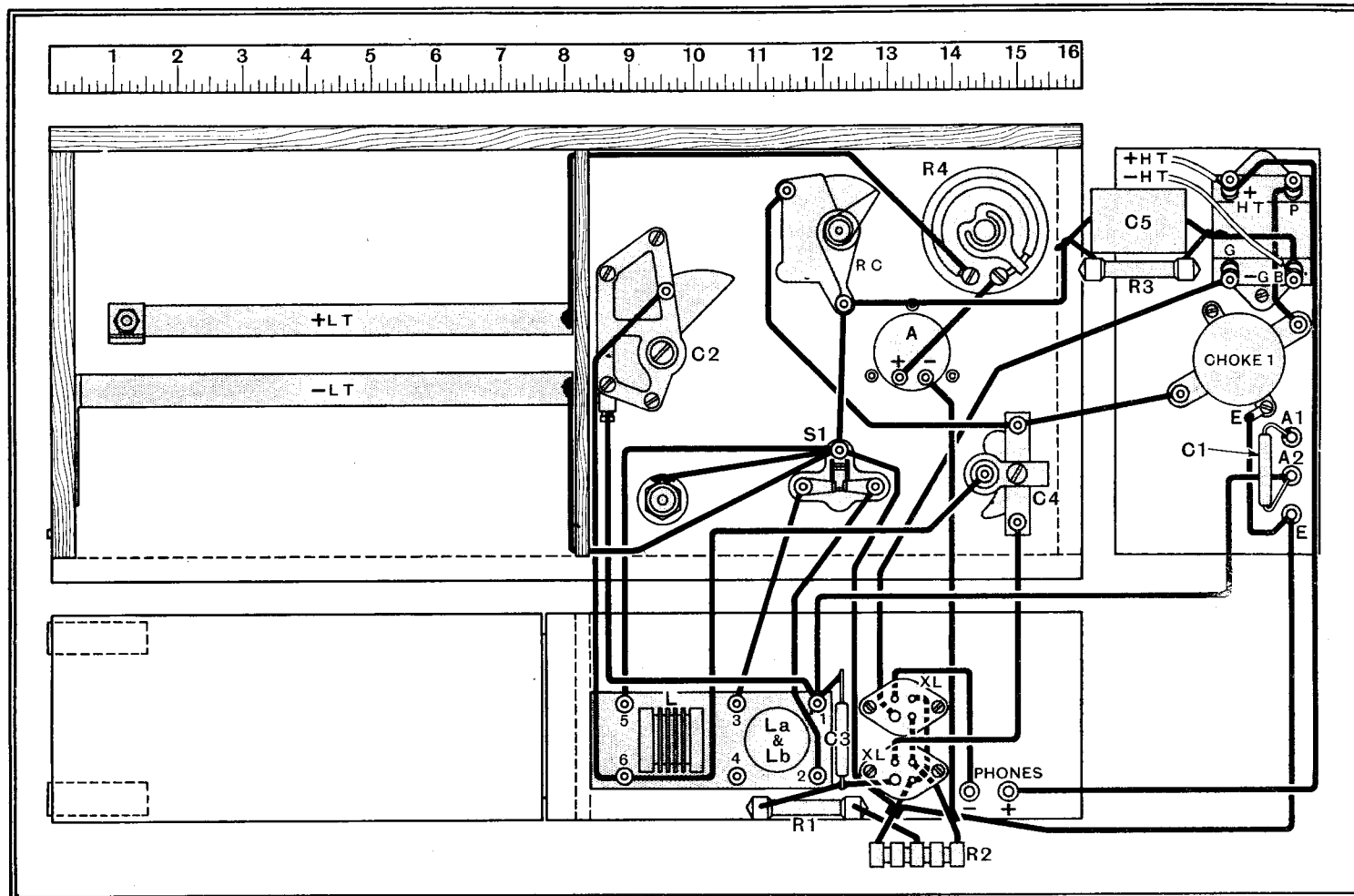
Practical wiring plan, with scale of inches for ascertaining dimensions and positions of components. Note that the bush of the slow-motion condenser drive knob (to the left of switch S1) is earthed. The inside back-to-front dimension of the cabinet is only 3\frac{1}{16} in.
