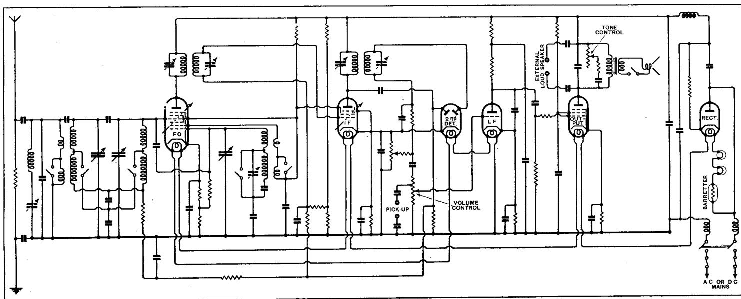
Complete circuit diagram. The pick-up, external loud speaker and aerial and earth connections are all isolated with condensers, and the mains leads include low-resistance HF chokes.
