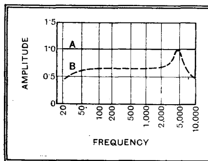
Fig. 2.—Showing the limitations in general output level resulting from a peaked response.
