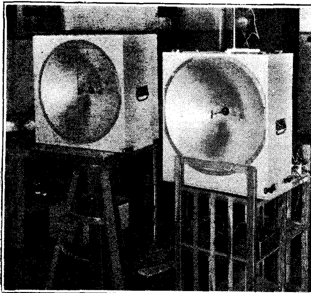
Ten-centimetre beam transmitter and receiver with reflectors.
