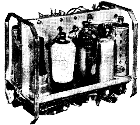
Chassis of Marconiphone car radio receiver.
