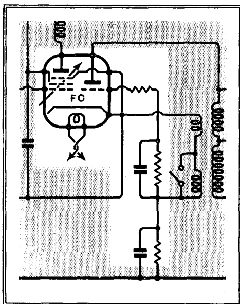
An advantage of the independent cathode; circuits of this kind are ruled out for battery valves.
