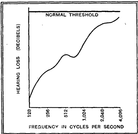
Fig. 7. Audiogram of person deaf to low frequencies.
