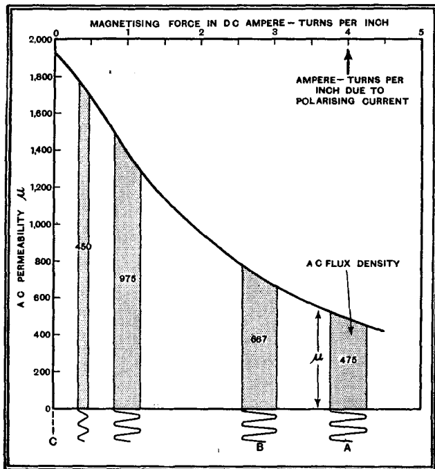
Fig. 1. Showing the fall in AC permeability when the core is polarised.
