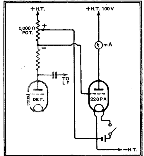
Circuit diagram of the indicator, showing connections to an existing receiver. Small voltage changes taking place in the anode circuit of a grid detector under the influence of an incoming signal are magnified, and cause easily discernible variations of the meter.
