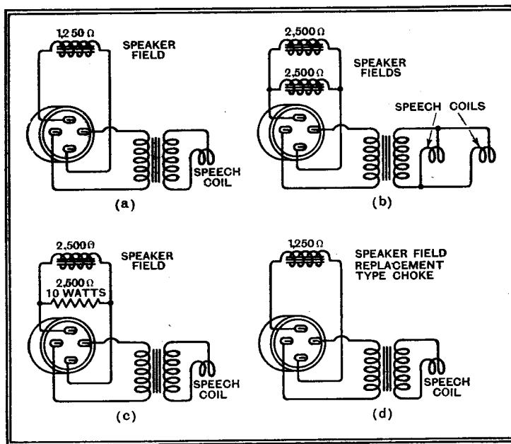
Fig. 1.—The connections between the loud speaker and the speaker-plug are shown at (a) for a 1,250-ohms field type, at (b) for dual speakers with 2,500-ohms fields, at (c) for a single 2,500-ohms field winding, and at (d) for a permanent magnet or separately energised speaker. As explained in the text, the connections of (c) are not always entirely satisfactory, since the resistance reduces smoothing.
