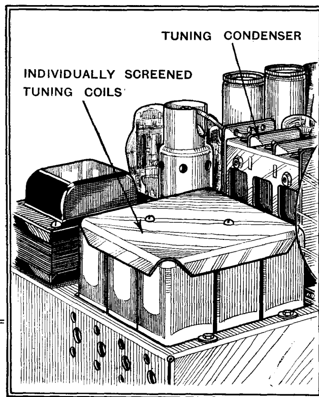
Individually screened coils are employed in this all-wave set in order to eliminate absorption spots.
