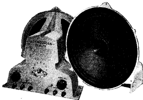
A "tweeter" unit is built into the centre pole piece of the Whiteley "Stentorian Duplex" loud speaker.
