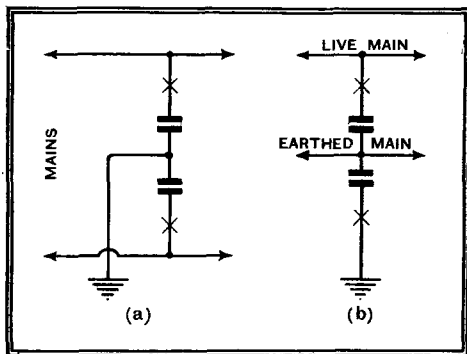
Fig. 1.—Two basic anti-interference filters; (a) is most suitable for DC and (b) for AC.
