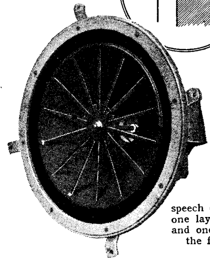
Large-diameter centring spider in the Sound Sales "Auditorium" loud speaker and (inset) special
