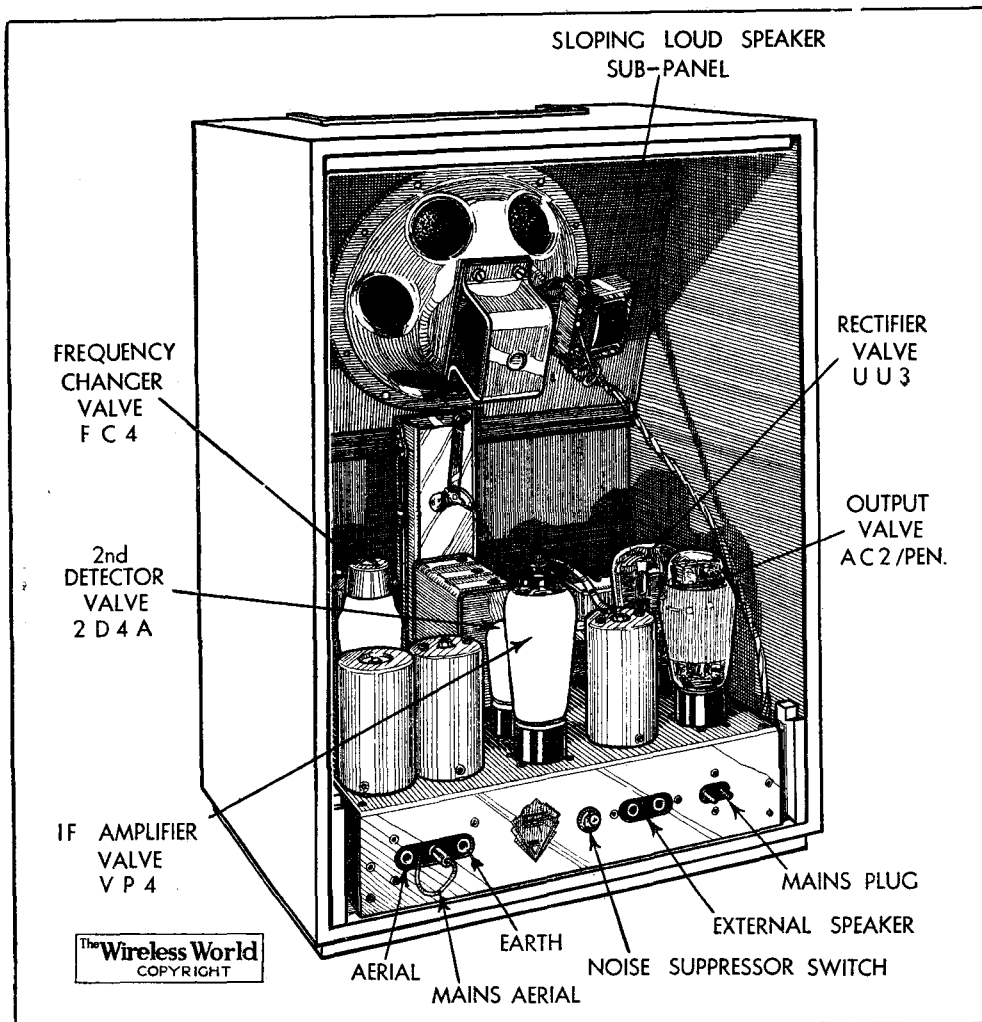
The chassis presents a particularly clean exterior appearance. Note the inclined loud speaker baffle.
