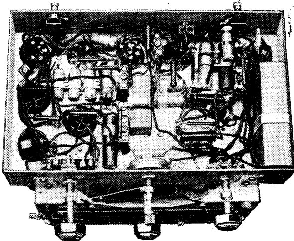
The components of the Ferranti Lancastria are arranged on the single-layer principle for accessibility, and are all firmly supported.
