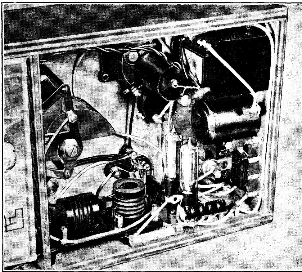
Although the receiver is compact there is no undue crowding of components. Note that the valve holders are raised on short distance-pieces.
