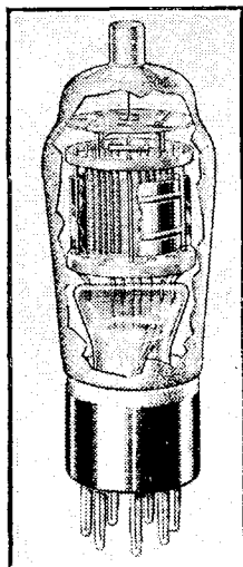
Mullard FC2 octode frequency-changer.
