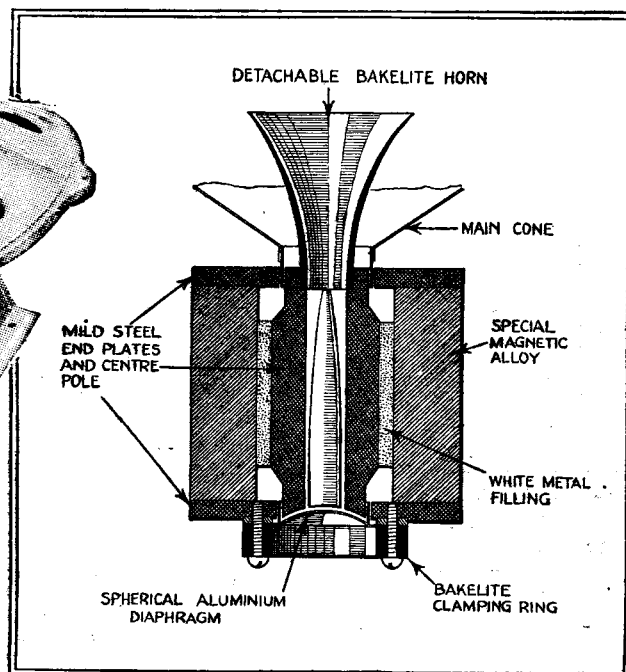
Whiteley "Stentorian Duplex" partly dismantled showing tweeter diaphragm. Note independent volume controls and output terminals. (Right) A section of "Stentorian Duplex" magnet system.
