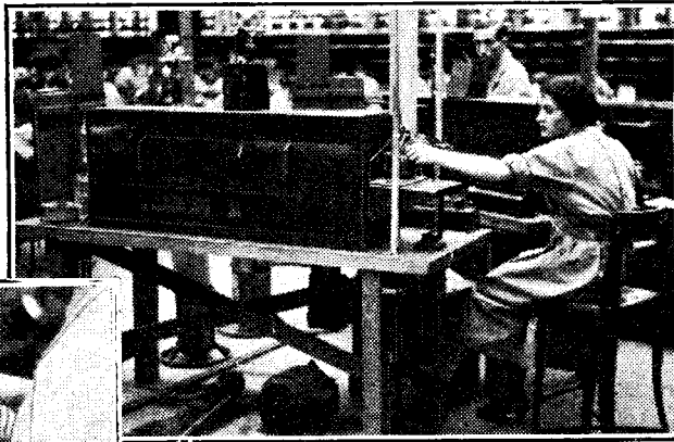
Resistance Making. (Right) One of the automatic electric furnaces for depositing the carbon surface. (Below) Spiral grinding machine for adjusting resistance value.
