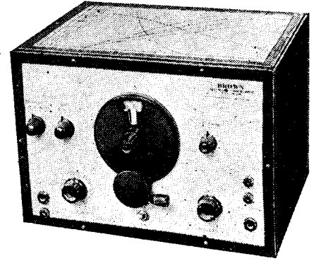
Brown All-wave modulated oscillator Type M2S.
