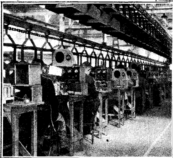
(Above) Assembling chassis and cabinets. Note the pneumatic hoists. (Left) General view of the test conveyor and benches.
