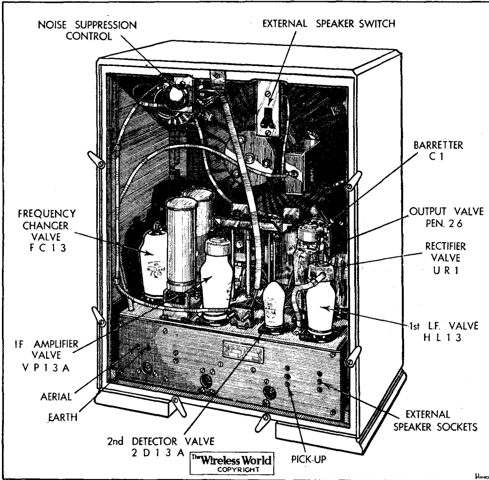
When the back of the set is removed the mains leads are automatically disconnected. Note the mains HF chokes behind the noise suppression control.
