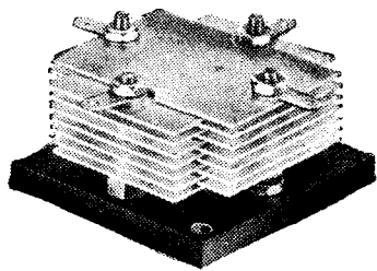
B.T.S. Air-dielectric Condenser.
