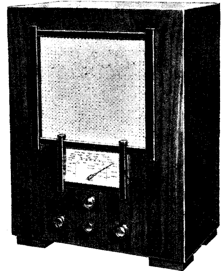
Climax battery receiver, Type MC36.
