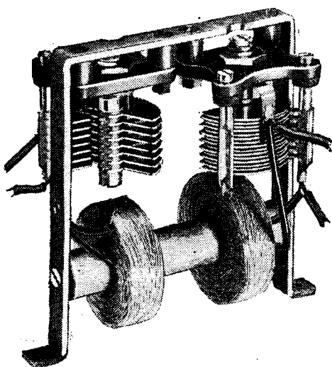
Litz-wound coils and air-spaced trimmers are used in the Eddystone 400/500 kc/s IF transformer.
