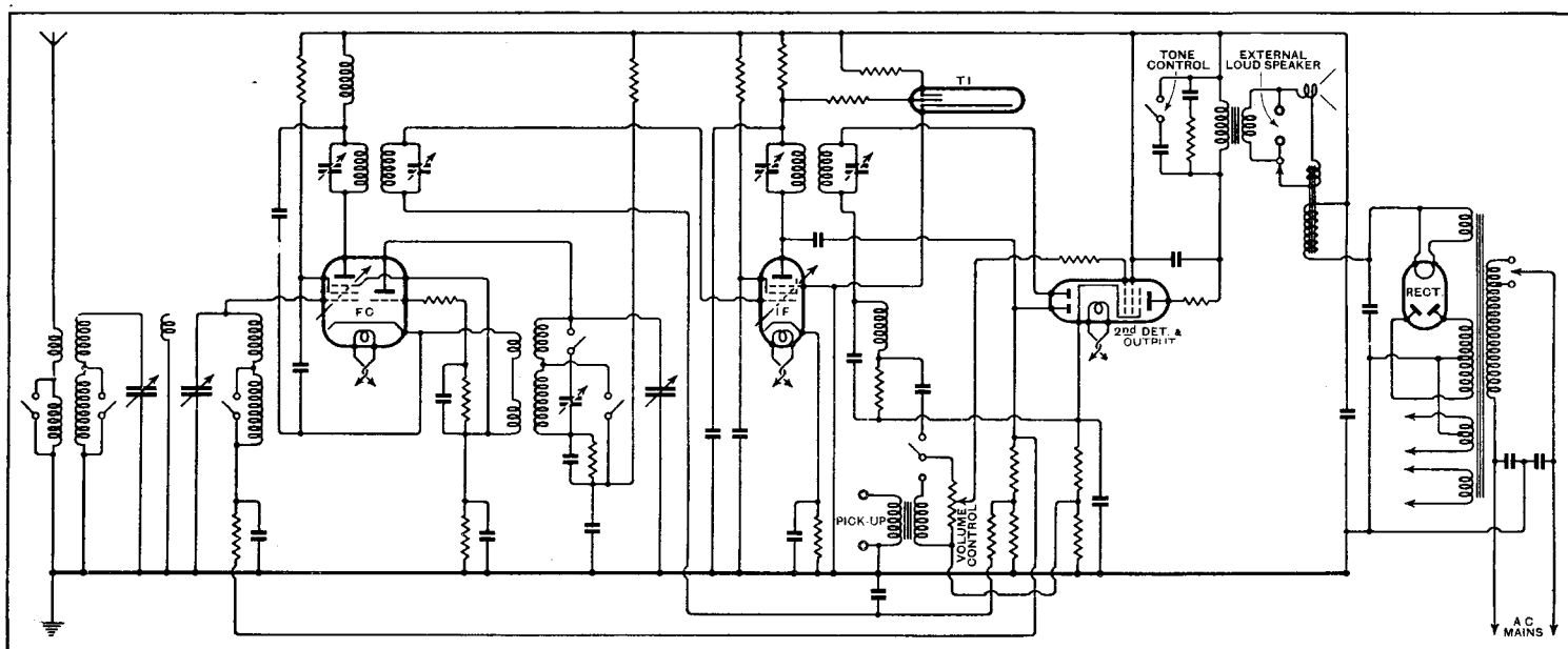
The three-valve circuit includes a combined detector-output valve, and an unusual refinement is the provision of a step-up input transformer for the pick-up.
